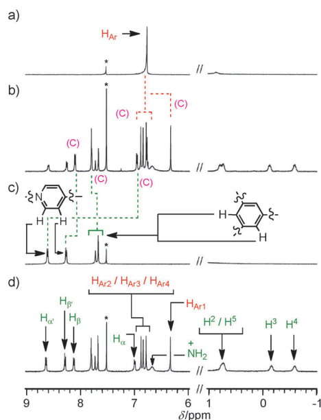
Figure 2. Partial 1 H NMR spectra (400 MHz, CDCl 3 /CD 3 CN (3:7), 298 K) of a) the molecular cage 1 , b) an equimolar mixture of 1 and the threadlike salt [2-H]2PF 6 (2 mM), c) [2-H]2PF 6 , and d) the [2]rotaxane [4-H]3PF 6 . In the spectrum in (b) the signals of protons in the complex are indicated by (C).
