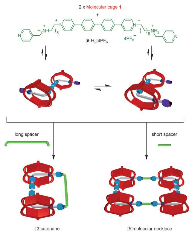
Scheme 2. Cartoon representation of the synthetic approach toward the [3]catenane and the [5]MN.
