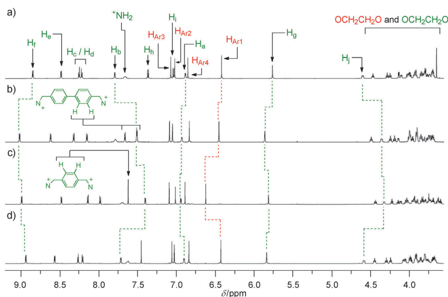
Figure 5. Partial ^1\text{H} NMR spectrum (800 MHz, \text{CD}_3\text{CN} , 298 K) of the [3]catenanes a) [7\text{-H}_2]6\text{PF}_6 , b) [9\text{-H}_2]6\text{PF}_6 , c) [10\text{-H}_2]6\text{PF}_6 , and d) the [5]MN [11\text{-H}_4]12\text{PF}_6 .
