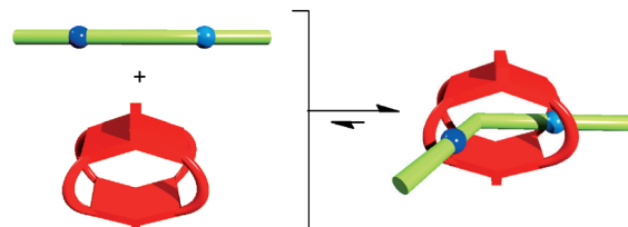
Figure 1. Cartoon representation of the precise folding of a linear guest within a cage-like host.
