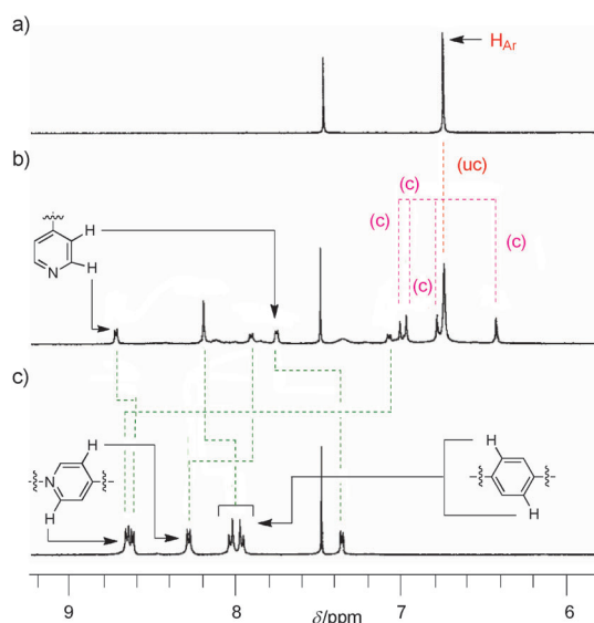
Figure 4. Partial ^1\text{H} NMR spectra (400 MHz, \text{CD}_3\text{CN}/\text{CDCl}_3 (1:1), 298 K) of a) the molecular cage 1 , b) a mixture of 1 (6 mM) and the threadlike salt [\mathbf{5}\text{-H}_2]\text{4PF}_6 (2 mM), and c) [\mathbf{5}\text{-H}_2]\text{4PF}_6 . In the spectrum in (b) the signals of protons in the complex are indicated by (c); (uc) stands for those of the uncomplexed molecule.
