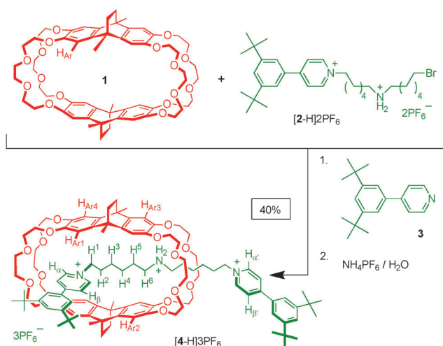
Scheme 1. Synthesis of the [2]rotaxane [4-H]3PF 6 .
