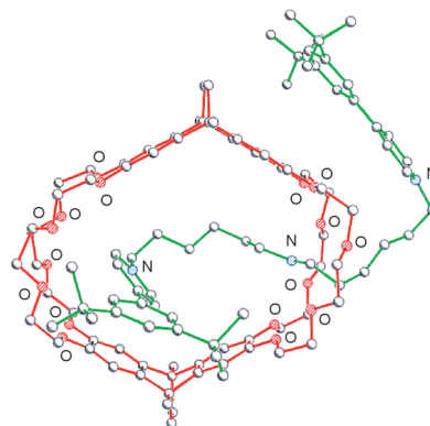
Figure 3. Ball-and-stick representation of the solid-state structure of the [2]rotaxane [4-H] 3+ .
