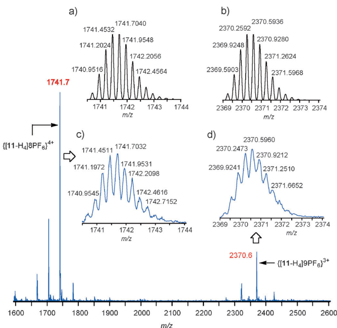
Figure 6. ESI mass spectrum of the [5]MN [11\text{-H}_4]12\text{PF}_6 exhibiting peaks corresponding to the molecular ions \{[11\text{-H}_4]8\text{PF}_6\}^{4+} and \{[11\text{-H}_4]9\text{PF}_6\}^{3+} and their calculated (a, b) and observed (c, d) isotopic distributions.
