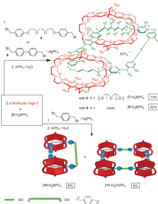
Scheme 3. Syntheses of three [3]catenanes and a [5]MN.
